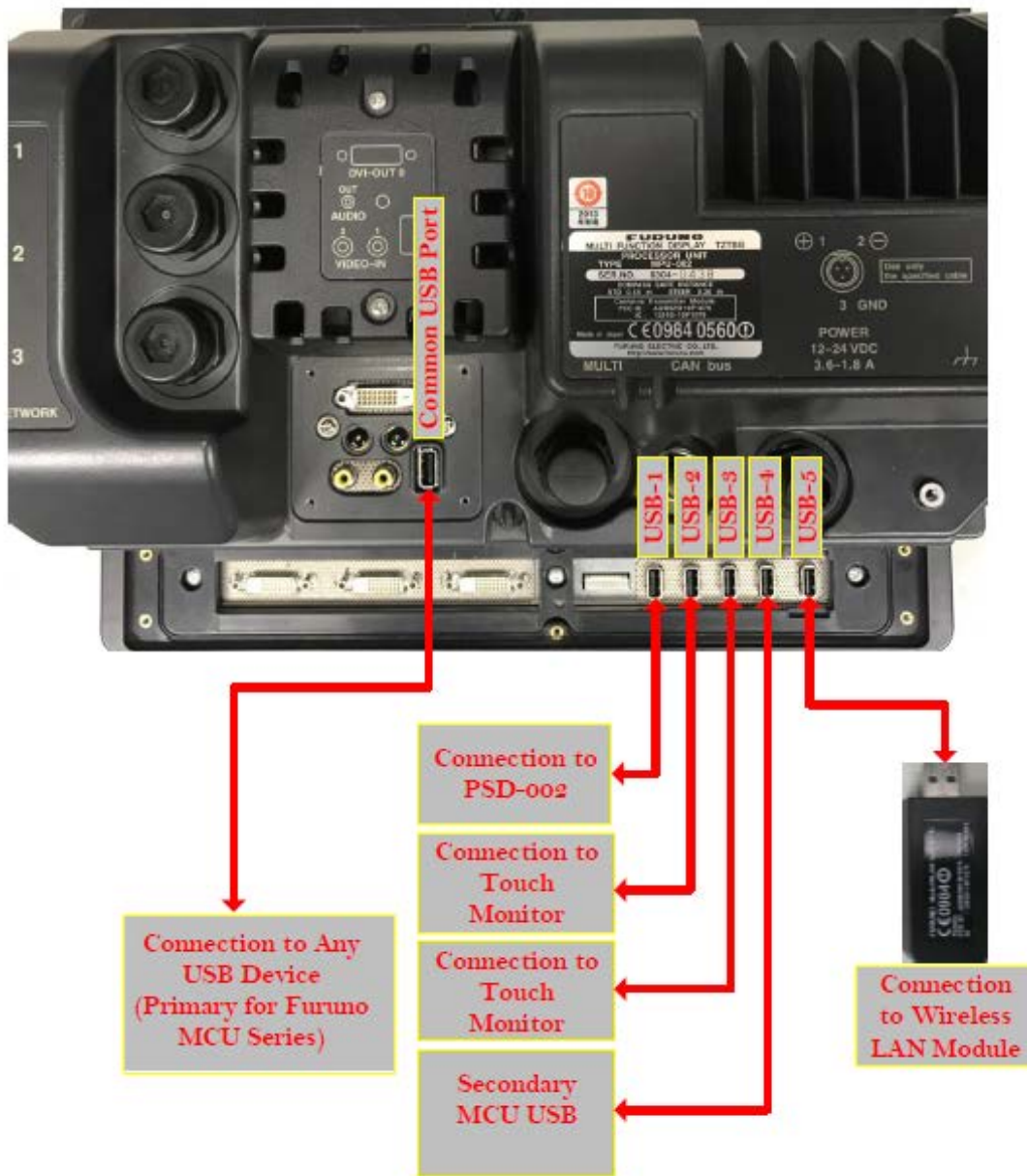
TZTBB processor shown, with USB port location and recommend usage
