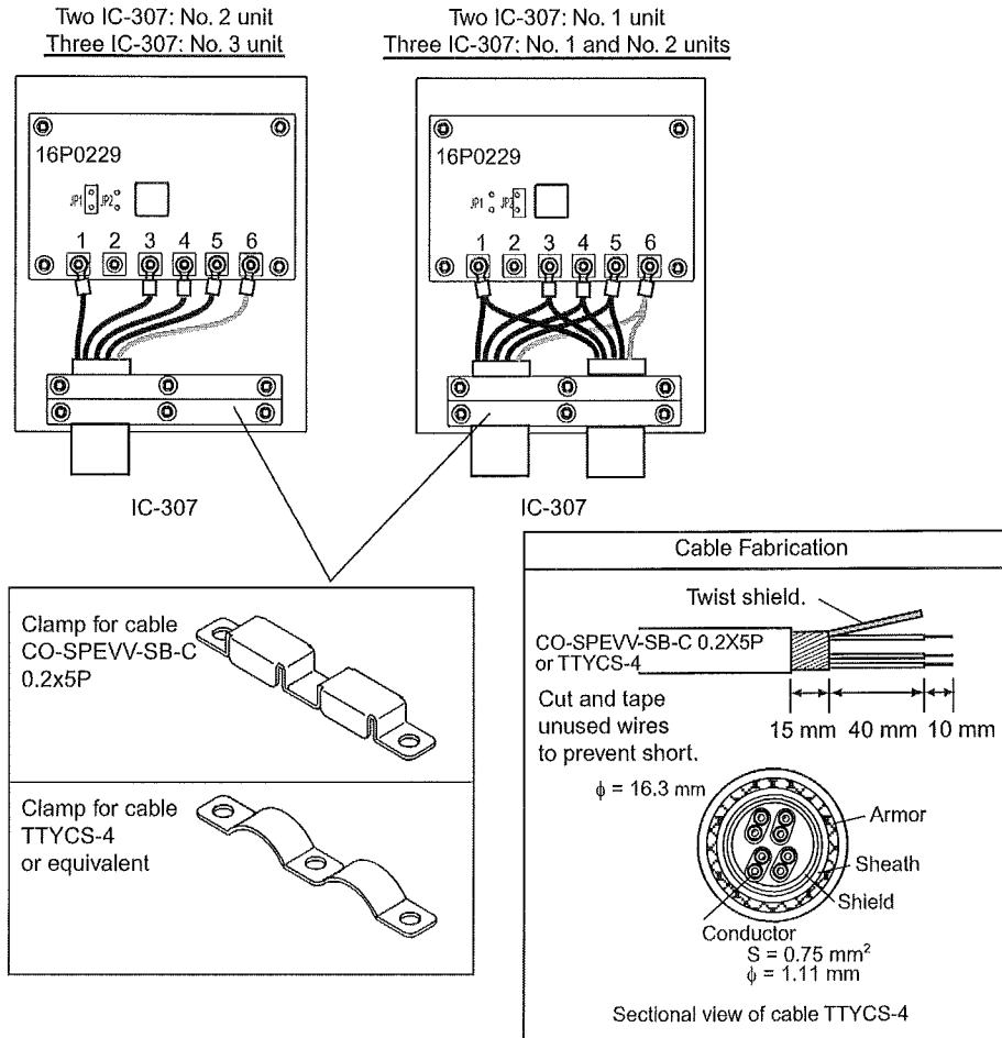
Wiring inside the SSAS alert unit
