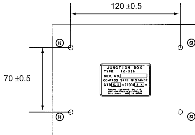
Junction box IC-315/318
