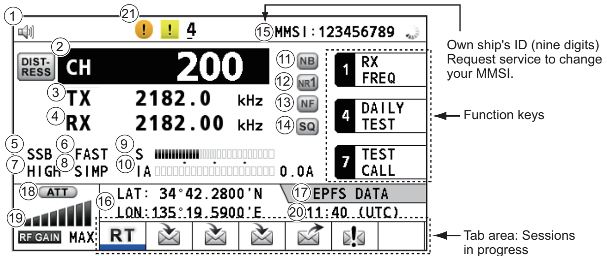
Radiotelephone (RT) screen
