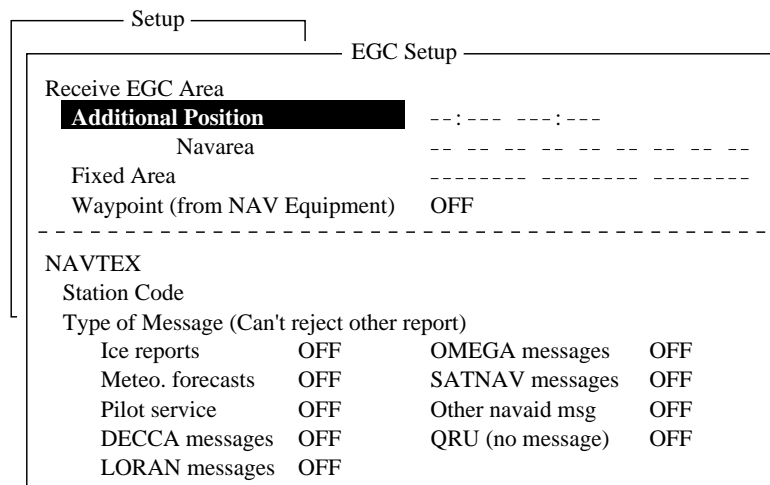
EGC setup menu
