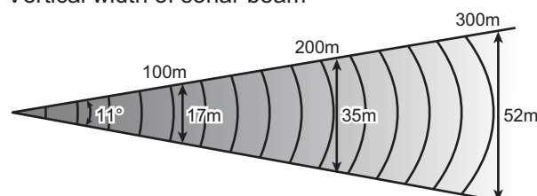
Vertical width of sonar beam
