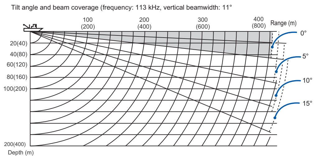
Vertical width of sonar beam
