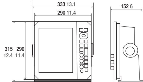
Display Unit model FR-10 3.2 kg 7 lbs
