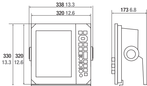
Display Unit model FR-10 3.2 kg 7 lbs
